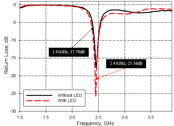
Fig. 8. Simulated result return loss, S_{11} without and with LED.
